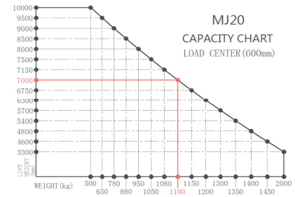
Capacity Chart-MJ20
