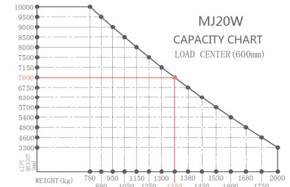
Capacity Chart-MJ20W
