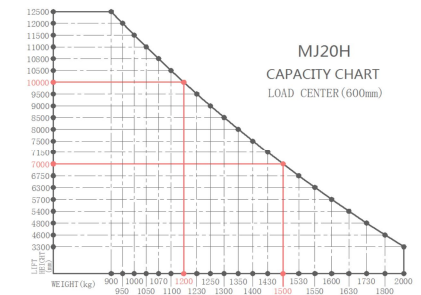
Capacity Chart-MJ20H
